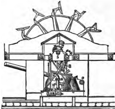
FIG. 181.—Oscillating Engine and Feathering Paddle-Wheel.
